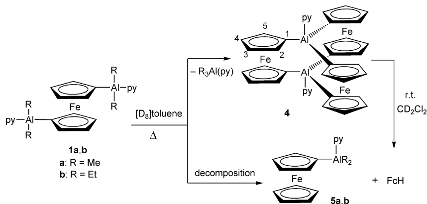
Scheme 5. Attempted synthesis of 4 and its decomposition.
