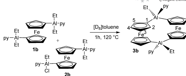
Scheme 4. Synthesis of ethylaluminum-bridged [1.1]ferrocenophane 3b .
