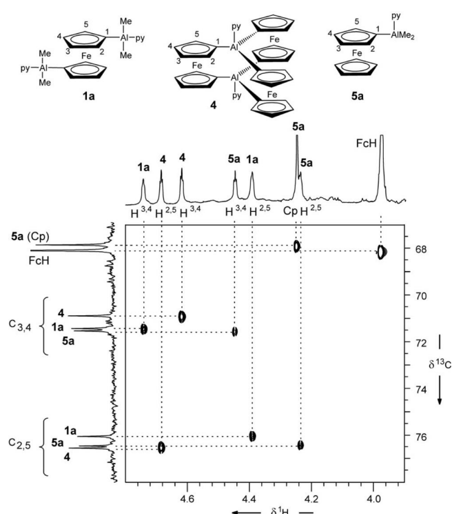
Figure 3. Contour plot of part of the 400 MHz 2D ^1\text{H} - ^{13}\text{C} -correlated spectrum (in [\text{D}_8]\text{toluene} at 23 °C) of a mixture containing 1a , 4 , 5a and ferrocene (after heating 1a with 2,2'-bipyridine for 2.5 h at 100 °C in [\text{D}_8]\text{toluene} ) recorded by the gradient-selected gHSQC method. [22]
