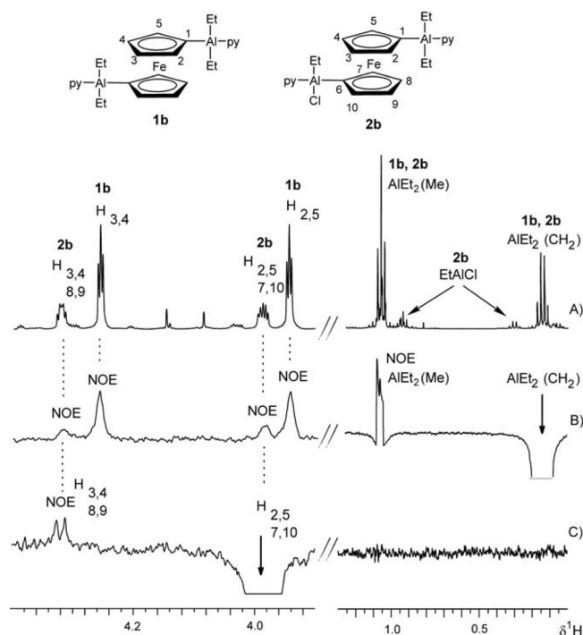
Figure 2. 400 MHz ^1\text{H} - ^1\text{H} gradient enhanced NOE difference spectra [21] of a mixture of 1b and 2b (in \text{CD}_2\text{Cl}_2 at 23 °C; relaxation delay 2.0 s; mixing time 0.6 s). The irradiated transitions are marked by arrows; the resulting intensities arising from NOE are indicated. The preferred solution-state conformations of 1b and 2b are shown. A) Normal ^1\text{H} NMR spectrum. B) Irradiation: \text{AlEt}_2 group of 1b ; response: ^1\text{H}_{2,5} and ^1\text{H}_{3,4} from 1b and ^1\text{H}_{2,5,7,10} and ^1\text{H}_{3,4,8,9} from 2b . C) Irradiation: ^1\text{H}_{2,5,7,10} from 2b ; response: ^1\text{H}_{3,4,8,9} from 2b .
