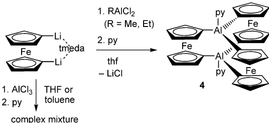
Scheme 6. Optimized synthesis of the trinuclear aluminum-bridged ferrocenophane 4 [best with \text{MeAlCl}_2 ; in the case of \text{EtAlCl}_2 , the formation of 3b was also observed (in repeated experiments with ca. 5–20%)].
