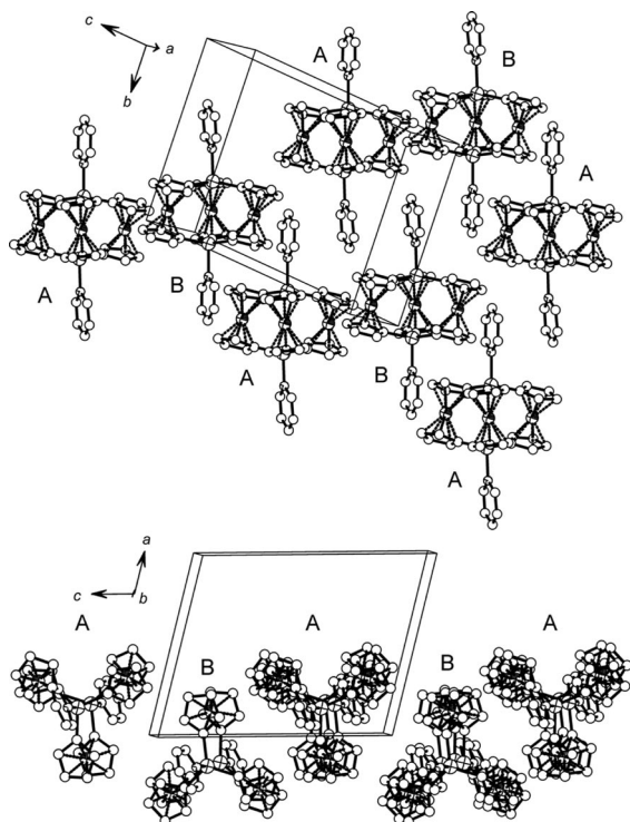
Figure 6. Two different views (see the axes systems) of the arrangements of the enantiomers A and B of 4 in the crystal lattice (the \text{CD}_2\text{Cl}_2 molecules are not shown).
