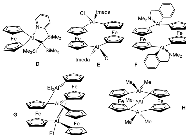
Scheme 2. Some aluminum compounds derived from 1,1'-disubstituted ferrocene; D , [11] E , [12a] F , [12b,15] G , [15] H . [16]
