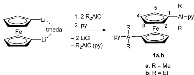
Scheme 3. Synthesis of the 1,1'-bis(dialkylalanyl)ferrocenes as dipyridine adducts [the stoichiometry of fcLi 2 (tmeda) is ill defined. Therefore, a slight excess amount of R 2 AlCl was used].
