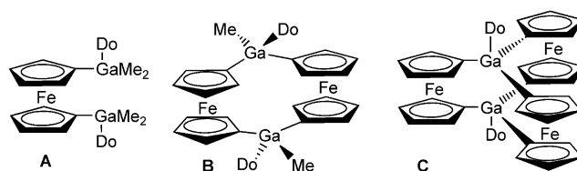
Scheme 1. Typical gallium compounds derived from 1,1'-disubstituted ferrocene; A , [17] B , [18a] C [19] (Do is, for example, pyridine or dmsol).
