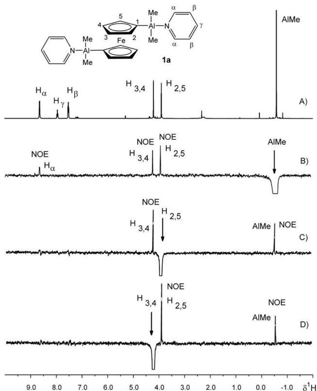
Figure 1. 400 MHz 1 H- 1 H gradient enhanced NOE difference spectra [21] of 1a (in CD 2 Cl 2 at 23 °C; relaxation delay 1.5 s; mixing time 0.8 s). Irradiated transitions are marked by arrows; the resulting intensities arising from NOE are indicated. The observed NOE for 1 H 3,4 upon irradiation of the 1 H(AlMe 2 ) transitions indicate that the structure shown for 1a is the preferred conformation. A) Normal 1 H NMR spectrum. B) Irradiation: 1 H(AlMe 2 ); response: 1 H 2,5 (larger) and 1 H 3,4 (smaller) and 1 H(H α -py). C) Irradiation: 1 H 2,5 ; response: 1 H 3,4 and 1 H(AlCH 3 ) of the Me 2 Al group. D) Irradiation: 1 H 3,4 ; response: 1 H 2,5 and 1 H(AlCH 3 ) of the Me 2 Al group.
