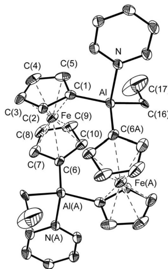
Figure 4. Molecular structure of 3b (ORTEF plot, 30% probabilities; hydrogen atoms are omitted for clarity; see Table 3 for structural parameters). The methyl carbon atoms of the ethyl groups are statistically disordered. This can be seen by the unusually large temperature coefficients (due to this disorder, the relevant C–C distances are too long).
