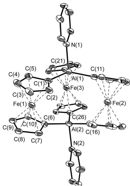
Figure 5. Molecular structure of 4 (ORTEP plot, 30% probabilities; hydrogen atoms are omitted for clarity; the \text{CD}_2\text{Cl}_2 molecules found in the crystal lattice are not shown; see Table 3 for structural parameters).
